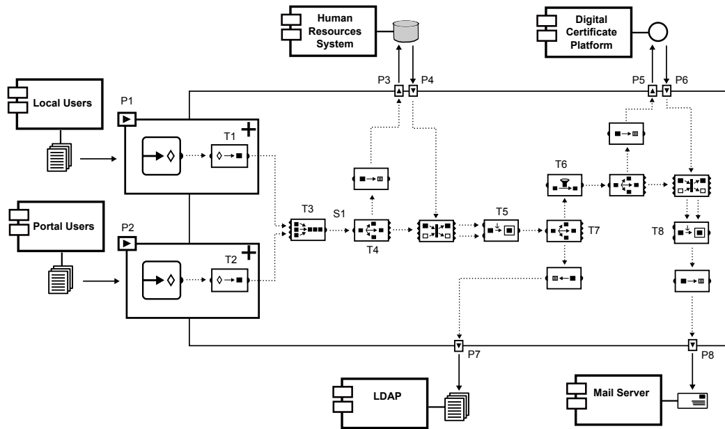
Figure 14: The integration solution conceptual model.
