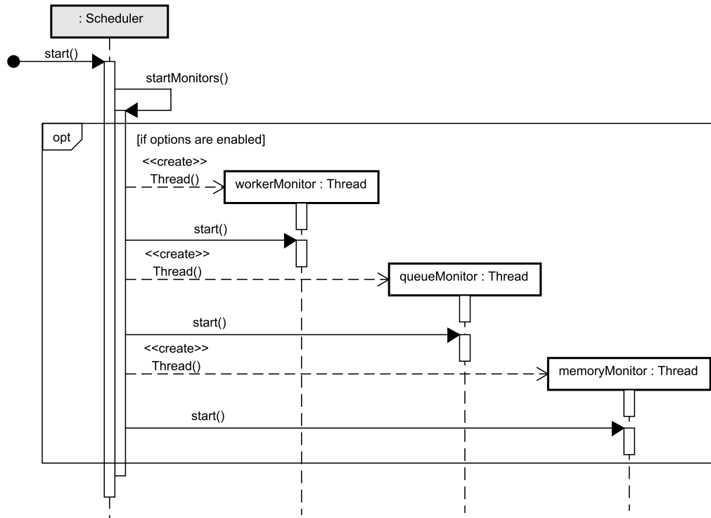
Figure 9: Creating and starting monitors.
