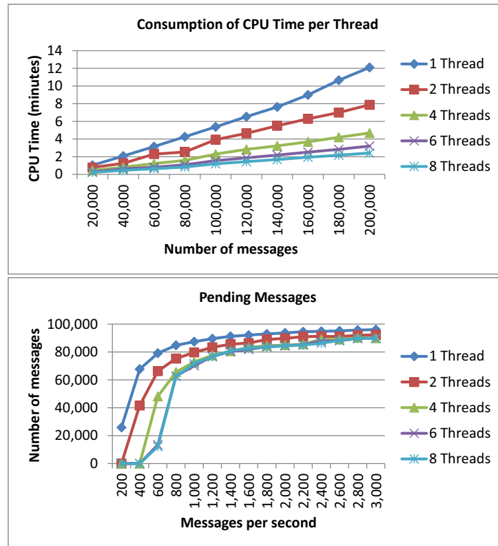
Figure 15: Experimental results for the integration solution.
