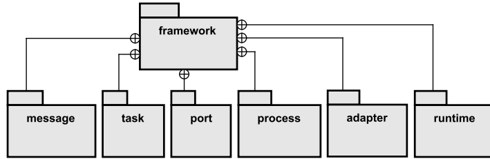
Figure 1: Packages of which our framework is composed.
