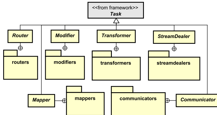
Figure 12: Task model in the toolkit.
