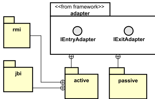
Figure 13: Adapter model in the toolkit.
