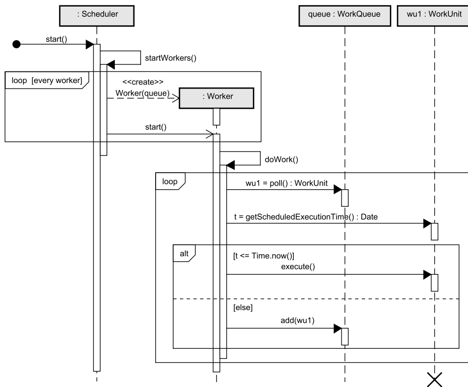
Figure 10: Creating and starting workers.
