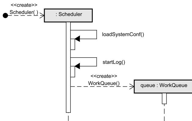
Figure 8: Initialising the Runtime System.
