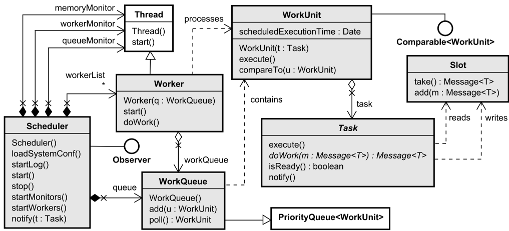
Figure 7: Task-based runtime model.
